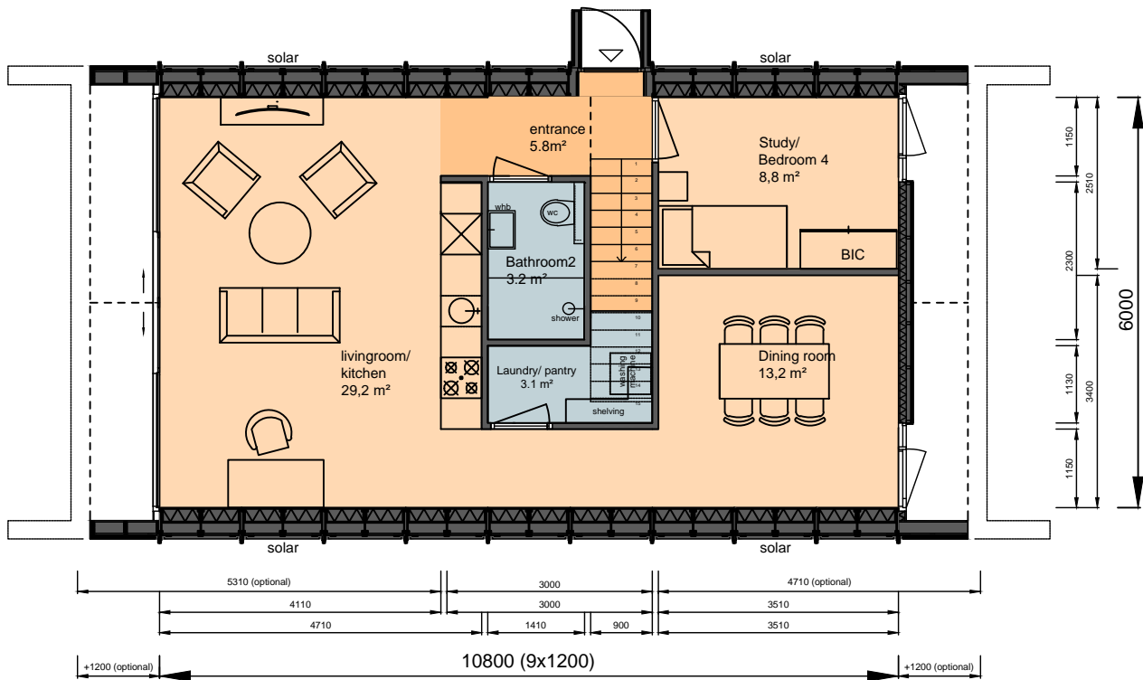
GROUND FLOOR
