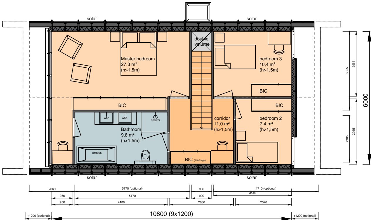
FIRST FLOOR
