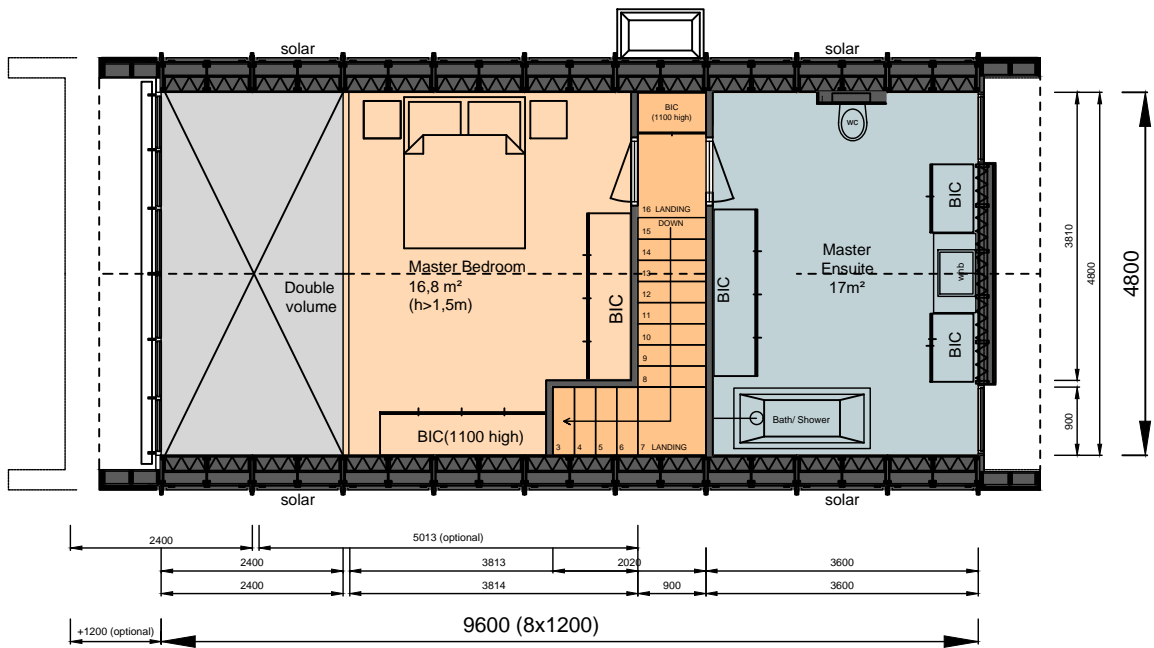
FIRST FLOOR
